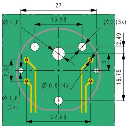
Figure 6: PCB Layout
